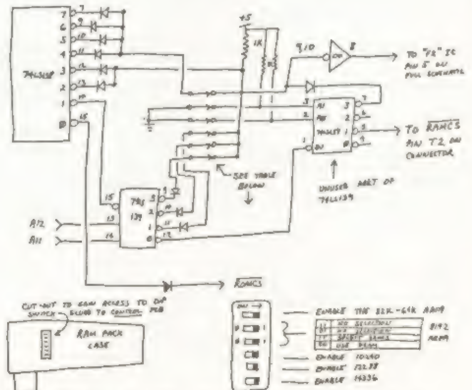
Figure 2: Optional RAM Pack Configuration Switch
